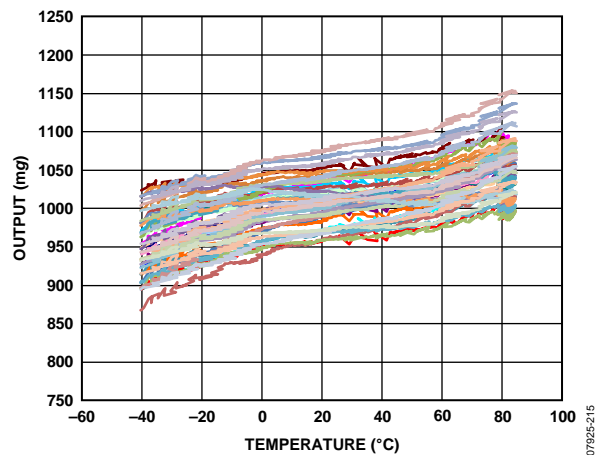
Figure 15. Z-Axis One g Offset vs. Temperature— 45 Parts Soldered to PCB, V_s = 2.5 V
