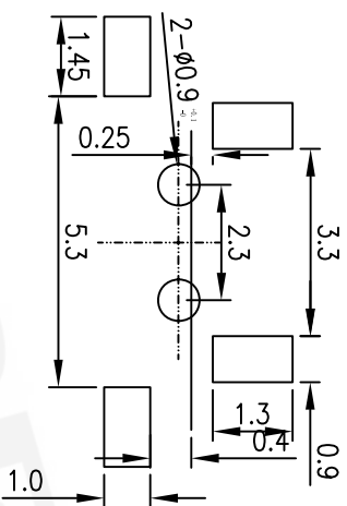
P.B.C BLAYOUT TOP VIEW
