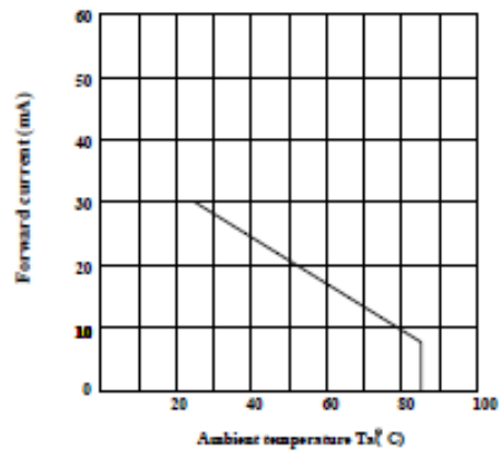
Forward current derating curve vs. ambient temperature
