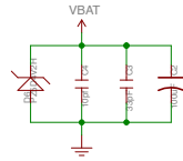
POWER DECOUPLING
